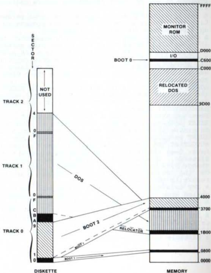
FIGURE 5.2 - BOOTSTRAP PROCESS
