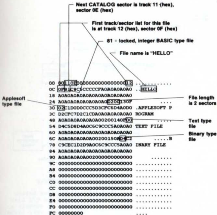
FIGURE 4.4 — EXAMPLE CATALOG SECTOR
