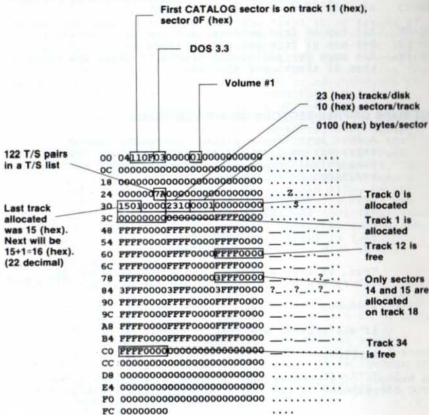
FIGURE 4.2 — EXAMPLE VTOC
